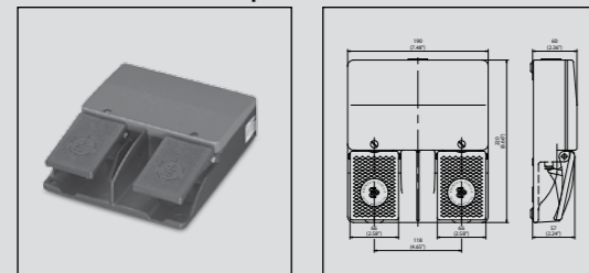
F2 – Foot switch with two pedals
