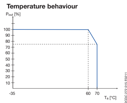
Characteristic curve of temperature at rated load
