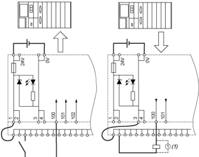
(1) Inductive load
