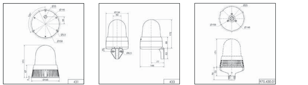
The adaptor enables mounting on a tube (accessory, only possible with base mounting 431)
